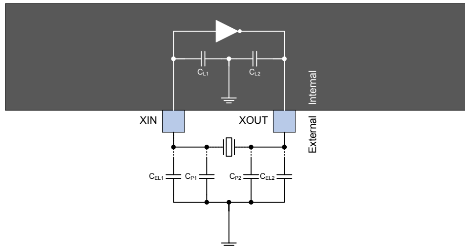
Figure 45-10. Crystal Circuit With Internal, External and Parasitic Capacitance
