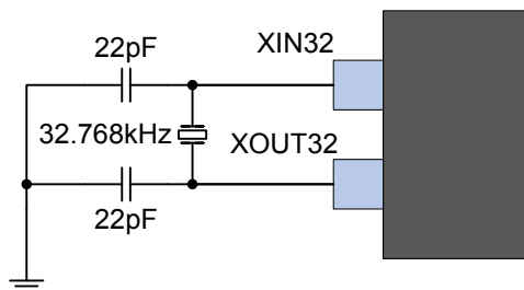
Figure 45-9. External Real Time Oscillator with Load Capacitor
