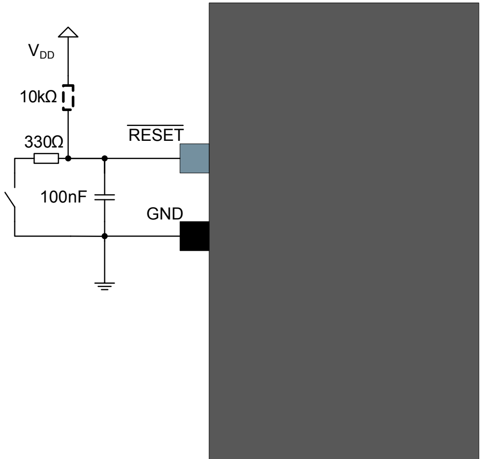
Figure 45-5. External Reset Circuit Schematic
