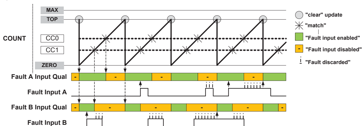
Figure 36-23. Fault Qualification in RAMP1 Operation
