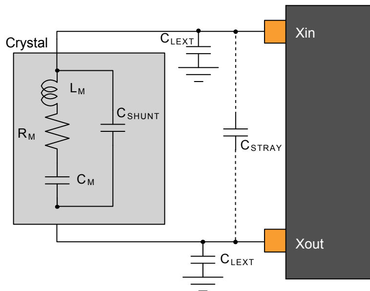
Figure 42-5. Oscillator Connection
