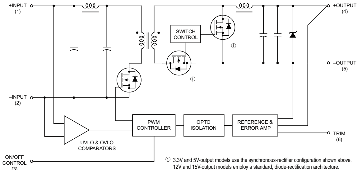
Figure 1. Simplified Schematic
