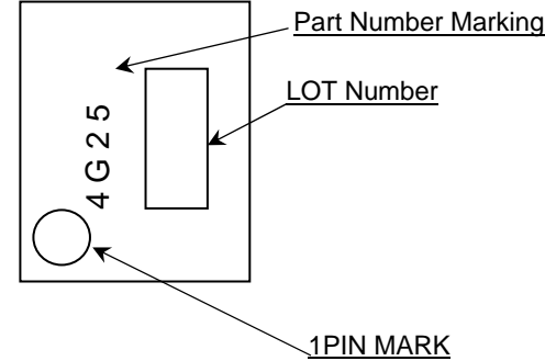
TSSOP-B8(TOP VIEW)
