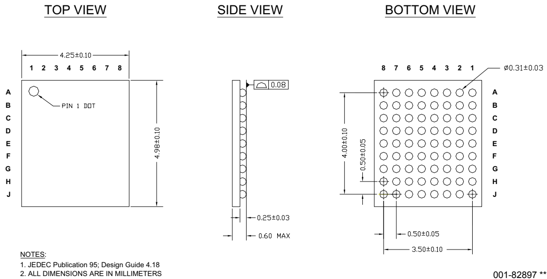
Figure 13-5. WLCSP Package ( 4.25 \times 4.98 \times 0.60 mm)
