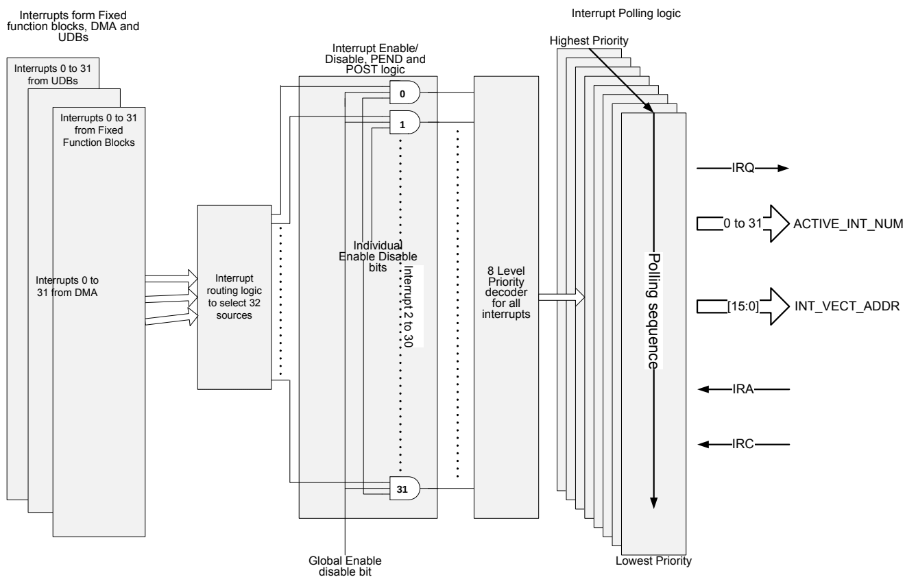
Figure 4-3. Interrupt Structure
