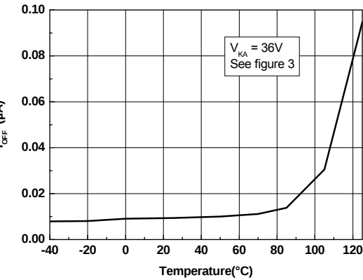
Figure 15. Off-state cathode current vs. temperature
