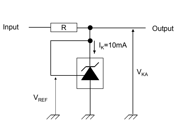
Figure 6. Test circuit V_{KA} = V_{REF}
