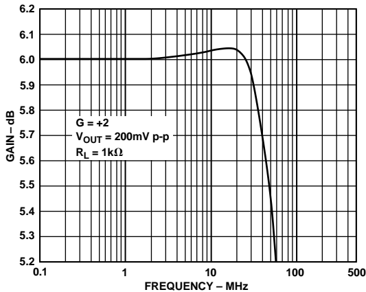
Figure 5. Gain Flatness; G = +2 ; V_S = \pm 5\text{ V} or +5\text{ V}
