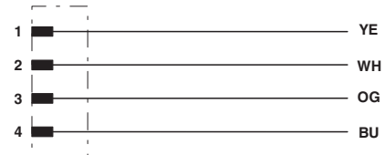
Circuit diagram
