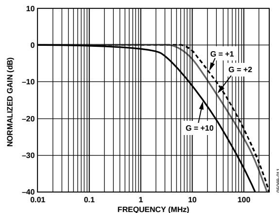
Figure 14. Large Signal Frequency Response for Various Gains ( V_S = \pm 5\text{ V} , V_O = 2\text{ V p-p} , R_L = 25\ \Omega )
