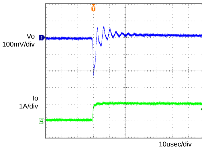
Figure 4. Transient Response (0→1.0A) Co=1\mu F, Ta=25^{\circ}C
