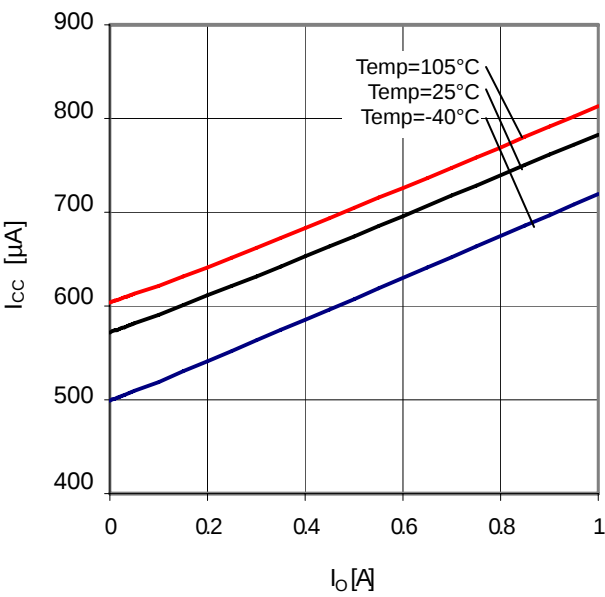
Figure 30. I_O-I_{CC}
