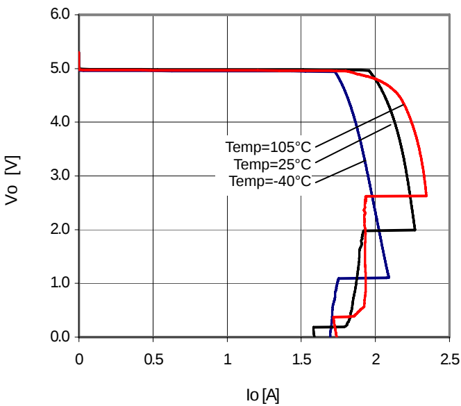
Figure 29. OCP
