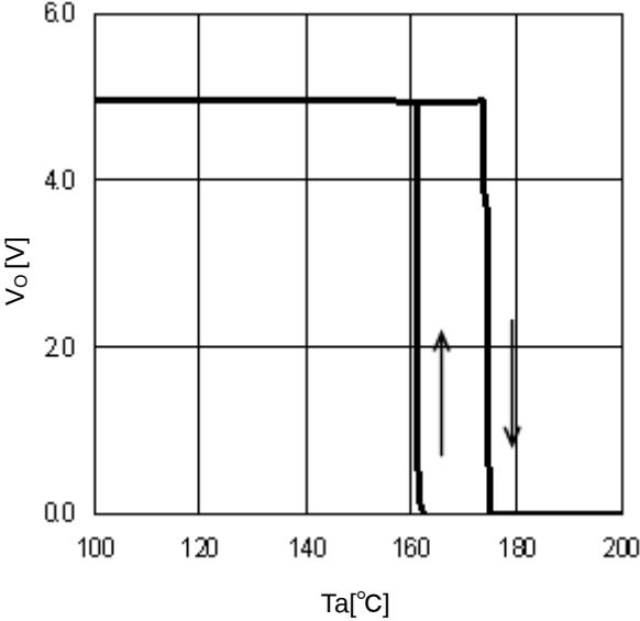
Figure 28. TSD ( I_O=0mA )
