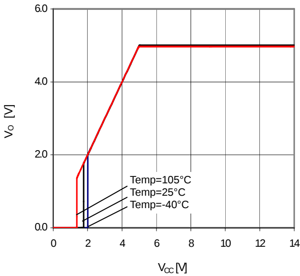
Figure 27. V_{CC}-V_O ( I_O=0mA )
