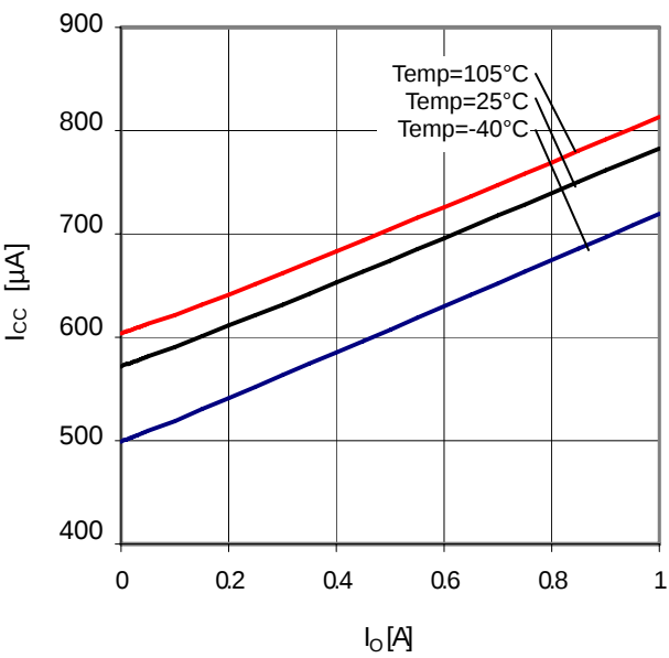
Figure 30. I_O-I_{CC}
