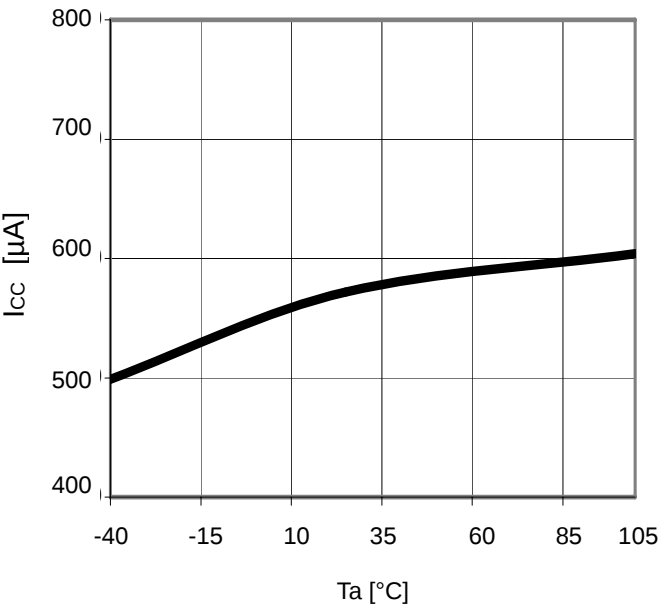
Figure 22. T_a - I_{cc}
