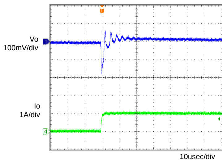
Figure 3. Transient Response (0→1.0A) C_o=1\mu F , T_a=-40^\circ\text{C}
