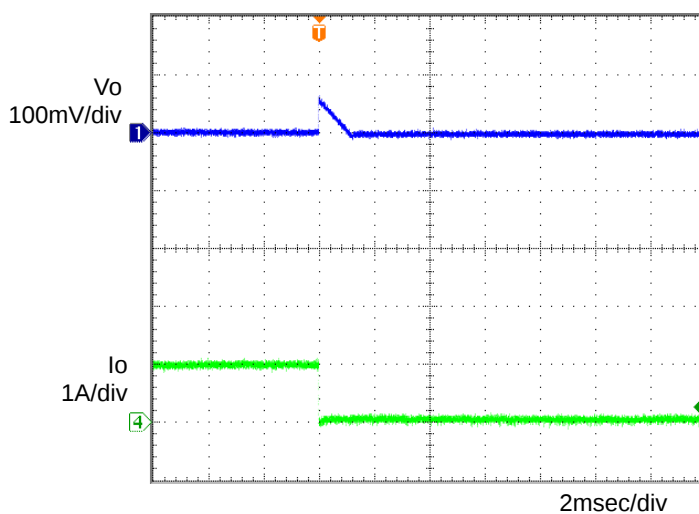
Figure 6. Transient Response (1.0→0A) C_o=1\mu F , T_a=-40^\circ\text{C}
