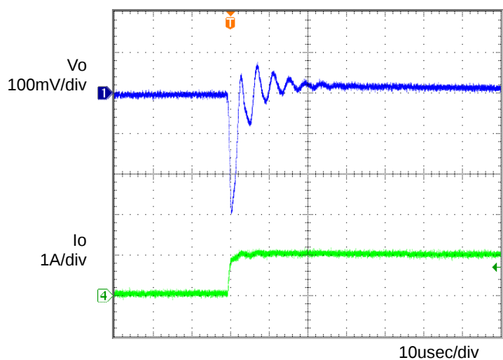
Figure 5. Transient Response (0→1.0A) C_o=1\mu F , T_a=105^\circ\text{C}
