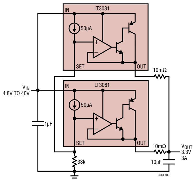
Figure 9. Parallel Devices
