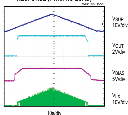
3.3V FIXED-OUTPUT SLOW V SUP RESPONSE (PWM, NO LOAD)
