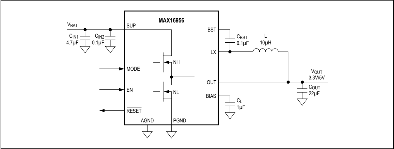
Figure 2. MAX16956AUBA/V+ (5.0V Fixed) and MAX16956AUBB/V+ (3.3V Fixed), 10-Pin μMAX
