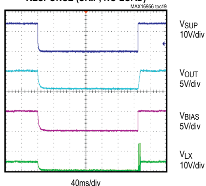
5V FIXED DIPS AND DROPS RESPONSE (SKIP, NO LOAD)
