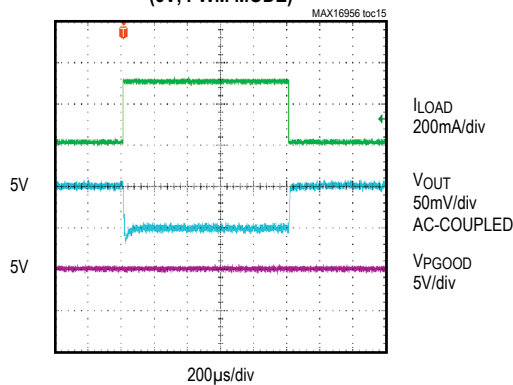
LOAD-TRANSIENT RESPONSE (5V, PWM MODE)
