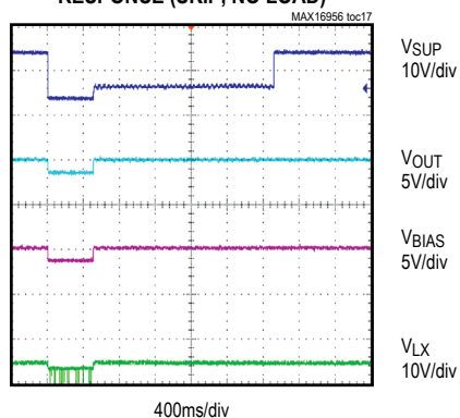
5V FIXED-OUTPUT COLD-CRANK RESPONSE (SKIP, NO LOAD)
