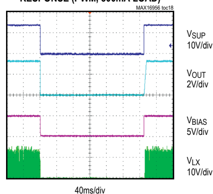
3.3V FIXED-OUTPUT DIPS AND DROPS RESPONSE (PWM, 300mA LOAD)
