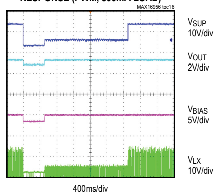
3.3V FIXED-OUTPUT COLD-CRANK RESPONSE (PWM, 300mA LOAD)
