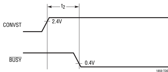
t 2 (CONVST to \overline{\text{BUSY}} Delay)
