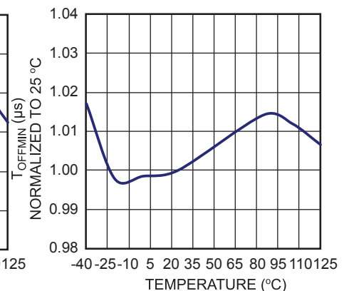
Minimum Off Time vs. Temperature
