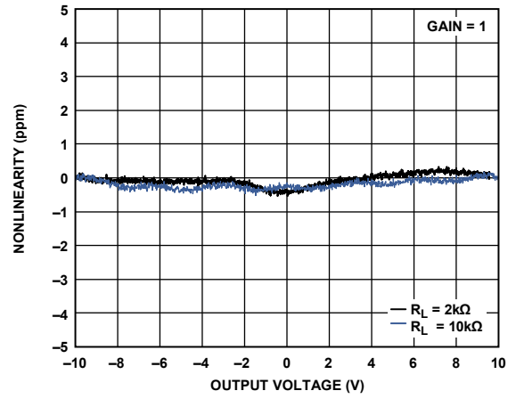
Figure 37. Gain Nonlinearity ( G = 1 ), R_L = 10\ \text{k}\Omega , 2\ \text{k}\Omega
