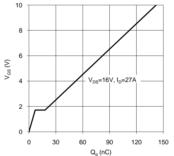
Figure 12. Gate Charge
