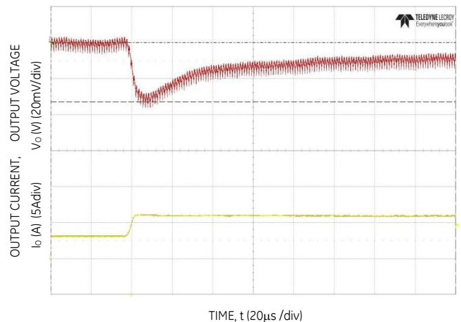
Figure 16. Transient Response to Dynamic Load Change from 50% to 100% at 12V in , C out =3x47μF+1x330μF, C Tune =3900pF, R Tune =300
