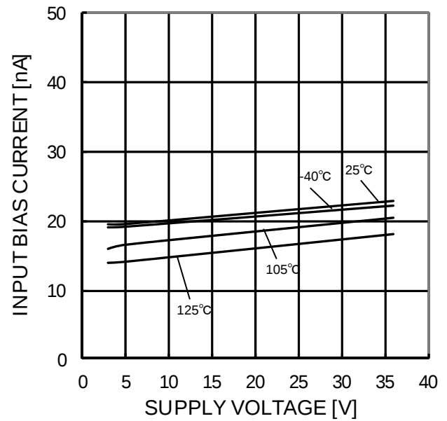
Figure 87. Input Bias Current - Supply Voltage ( V_{ICM}=0V , OUT=1.4V )
