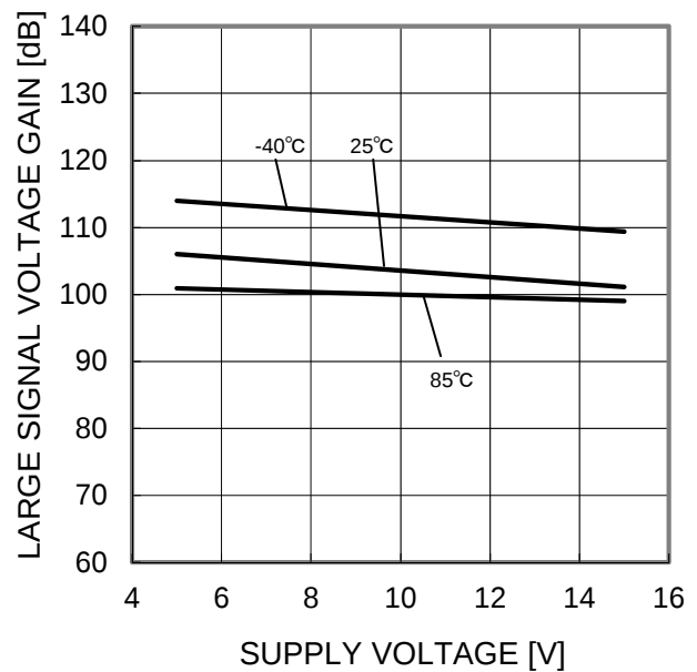
Figure 21. Large Signal Voltage Gain - Supply Voltage (R L =2kΩ)
