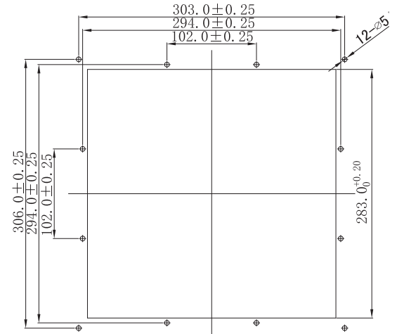
PANEL CUTOUT
