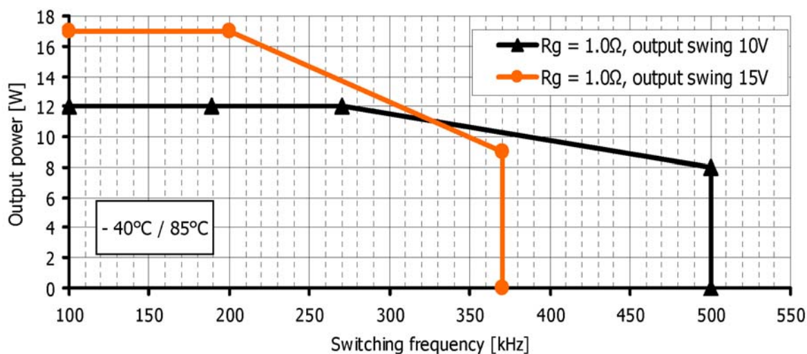
Fig. 4 Output power vs. switching frequency for ambient temperature range – 40°C through 85°C
