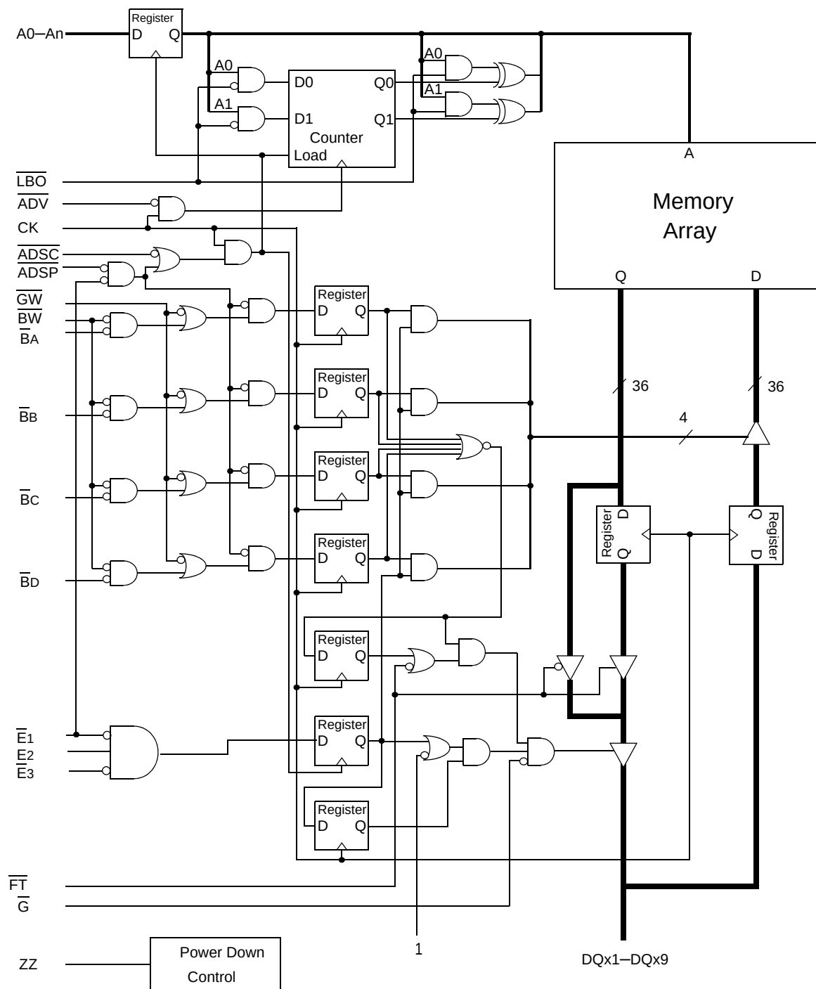
GS832118/32/36AD-xxxV Block Diagram
