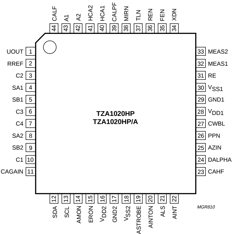
Fig.2 Pin configuration.
