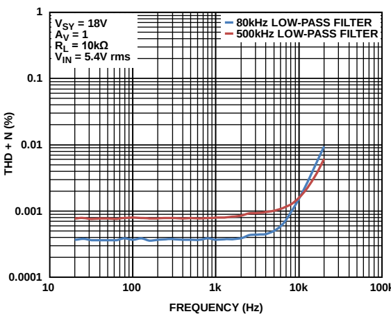
Figure 65. THD + N vs. Frequency
