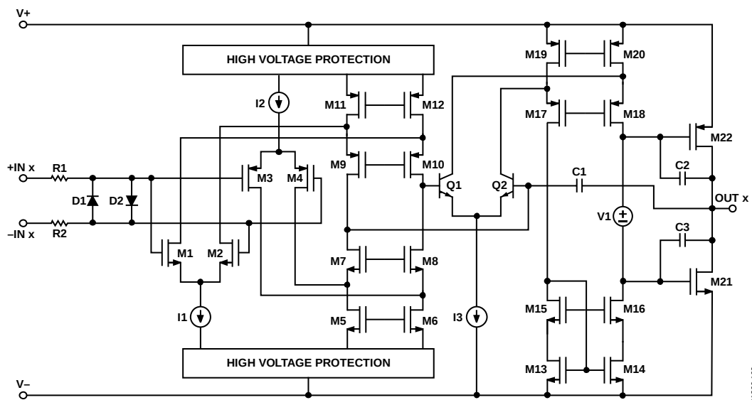
Figure 70. Simplified Schematic
