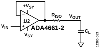
Figure 83. Stability Compensation with Isolating Resistor, R_{ISO}
