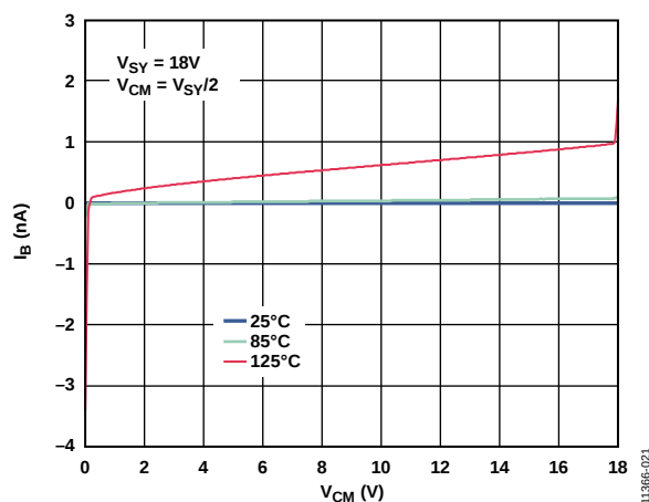
Figure 22. Input Bias Current vs. Common-Mode Voltage
