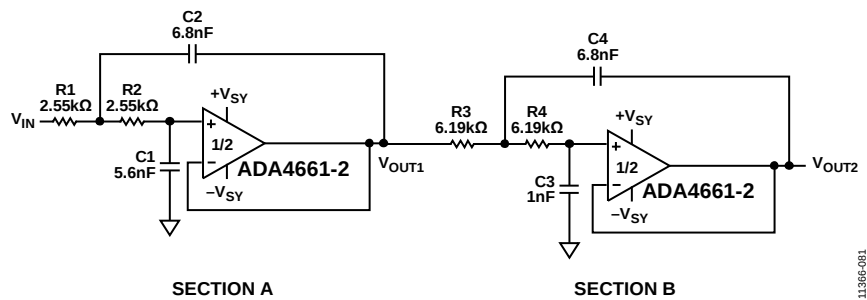
Figure 81. Four-Pole Low-Pass Filter
