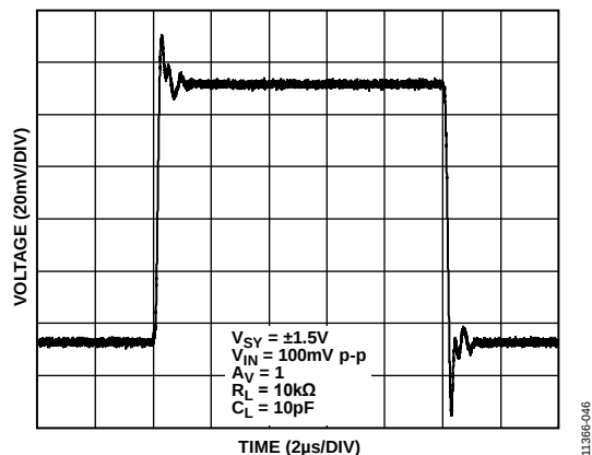
Figure 48. Small Signal Transient Response
