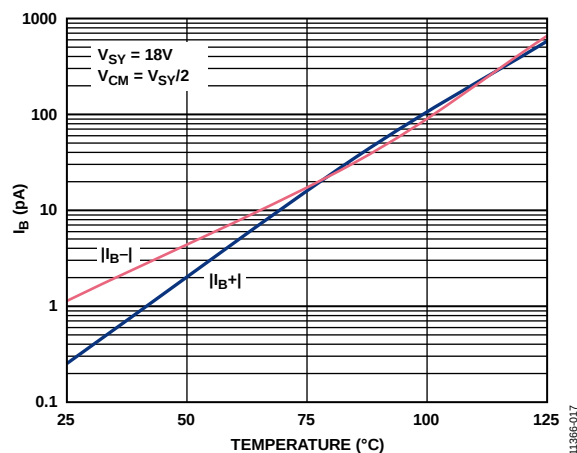
Figure 21. Input Bias Current vs. Temperature
