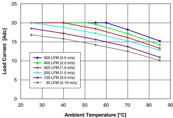
Fig. 1 : Available load current vs. ambient air temperature and airflow rates for converter with G height pins mounted vertically with air flowing from pin 1 to pin 3, MOSFET temperature \leq 125^{\circ}\text{C} , V_{in} = 48\text{ V} .
