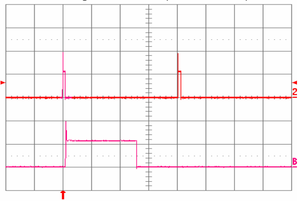
Fig. 16: Load current (top trace, 20 A/div., 50 ms/div.) into a 10 m \Omega short circuit during restart, at V_{in} = 48 V. Bottom trace (20 A/div., 2 ms/div.) is an expansion of the on-time portion of the top trace.
