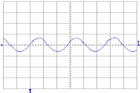
Fig. 11: Output voltage ripple (50 mV/div.) at full rated load current into a resistive load with C_o = 10\text{ }\mu\text{F} tantalum + 1 \mu\text{F} ceramic and V_{in} = 48\text{ V} . Time scale: 1 \mu\text{s} /div.
