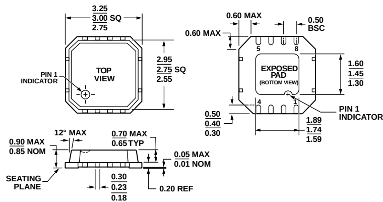
Figure 44. 8-Lead Frame Chip Scale Package [LFCSP_VD] 3 mm \times 3 mm Body, Very Thin, Dual Lead (CP-8-2)
