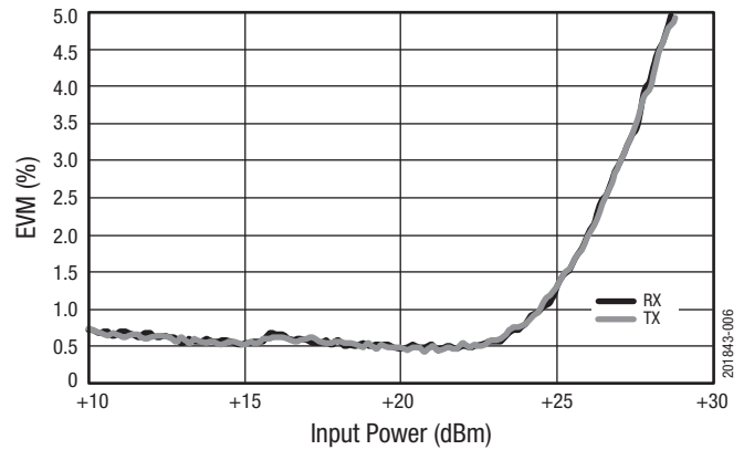
Figure 6. EVM vs Input Power (@ 2.45 GHz, 54 bps)
