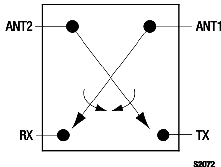
Figure 1. SKY13355-374LF Block Diagram
