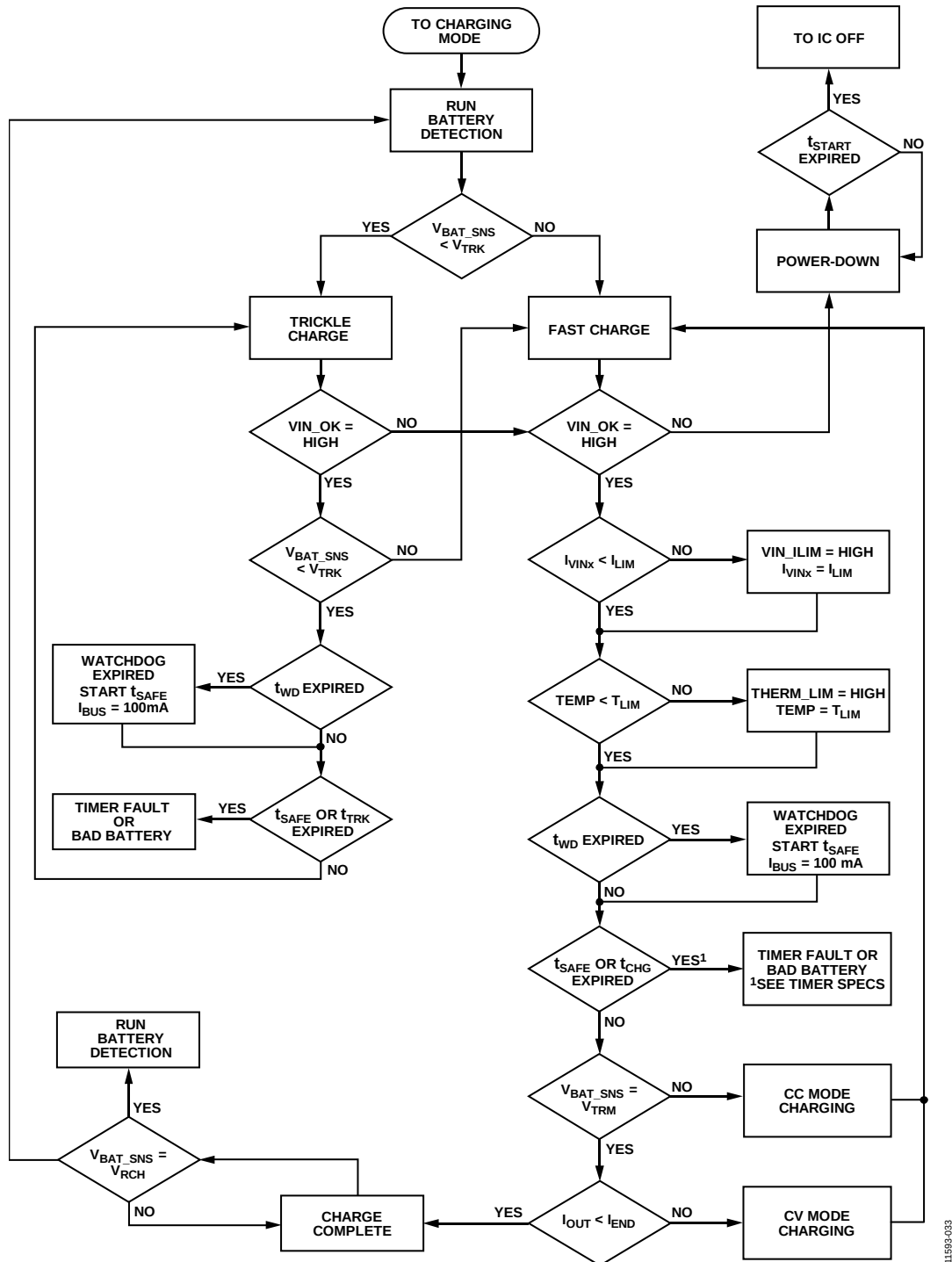
Figure 30. Simplified Charging Mode Flowchart
