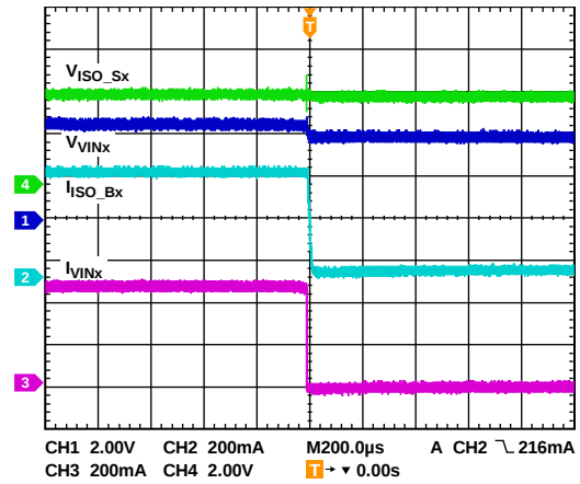
Figure 23. USB VBUS Disconnection
