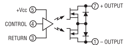
Figure 6 - Simplified Circuit
