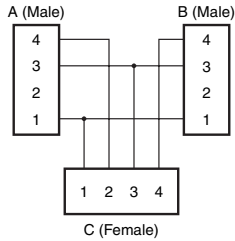
Wiring Diagram
