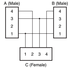
Wiring Diagram
