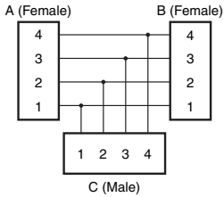
XS2R-D422-5
