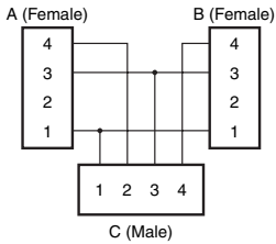
XS2R-D422-5
