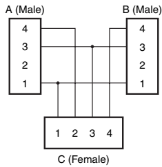
Wiring Diagram
