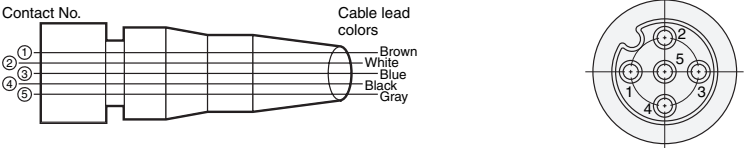
Wiring Diagram
