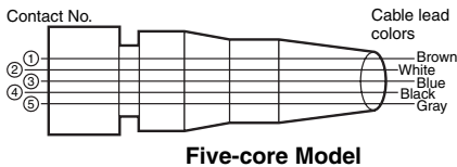
Five-core Model
