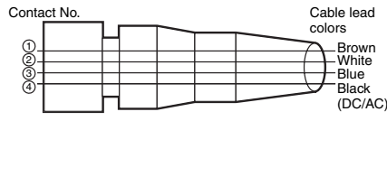
Four-core Model
