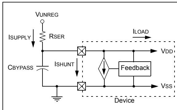
FIGURE 18-1: SHUNT REGULATOR
