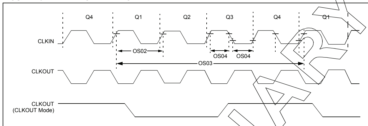
FIGURE 20-4: CLOCK TIMING
