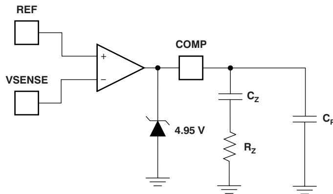
Figure 26. Typical Error Amplifier Compensation
