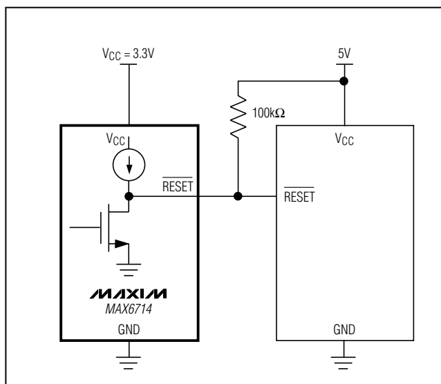
Figure 9. Interfacing to Different Logic Supply Voltage
