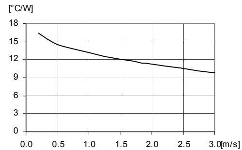
Thermal resistance vs. airspeed measured at the converter. Tested in wind tunnel with airflow and test conditions as per the Thermal consideration section.
