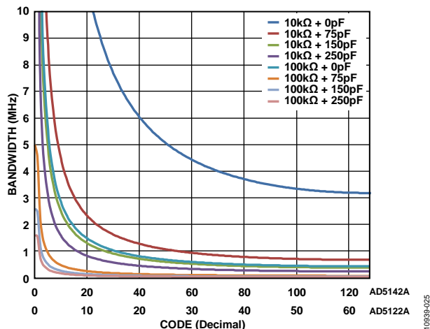
Figure 25. Maximum Bandwidth vs. Code and Net Capacitance
