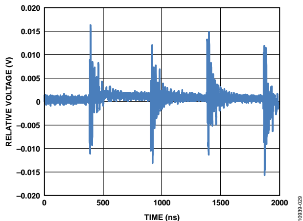
Figure 29. Digital Feedthrough
