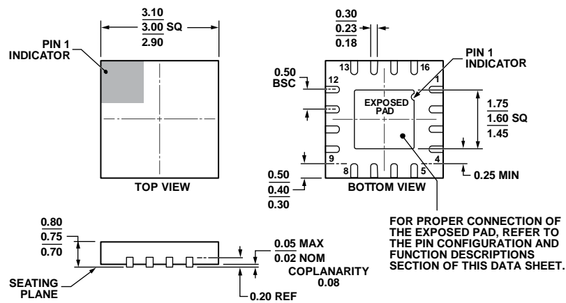
Figure 42. 16-Lead Lead Frame Chip Scale Package [LFCSQ_WQ] 3 mm × 3 mm Body, Very Very Thin Quad (CP-16-22)
