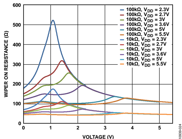
Figure 24. Incremental Wiper On Resistance vs. V_{DD}
