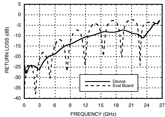
Data Output Return Loss vs. Frequency [1][3][4]
