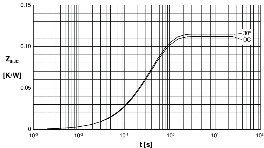
Fig. 8 Transient thermal impedance junction to case (per thyristor)
