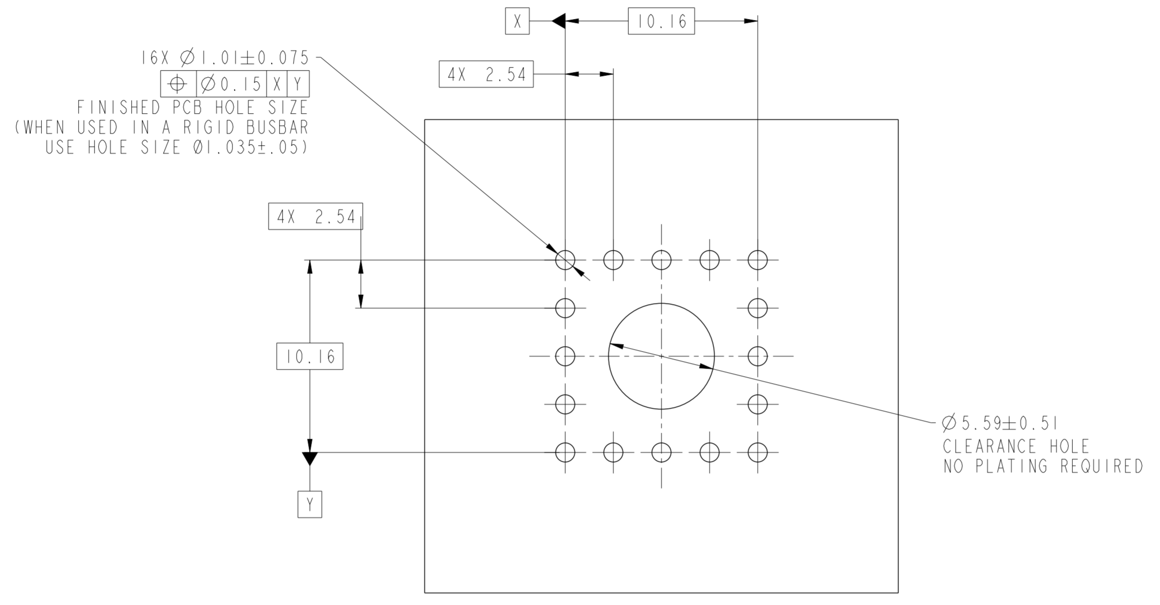
RECOMMENDED PCB BOARD LAYOUT
