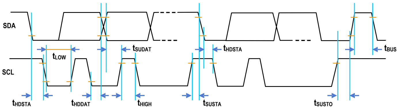
Figure 13. Timing Diagram
