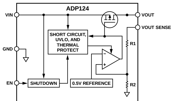
Figure 28. ADP124 Internal Block Diagram (Fixed Output)
