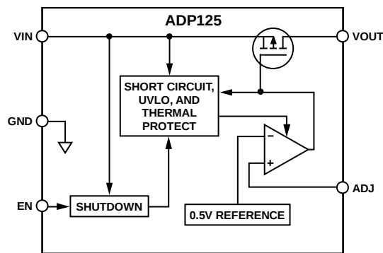
Figure 29. ADP125 Internal Block Diagram (Adjustable Output)
