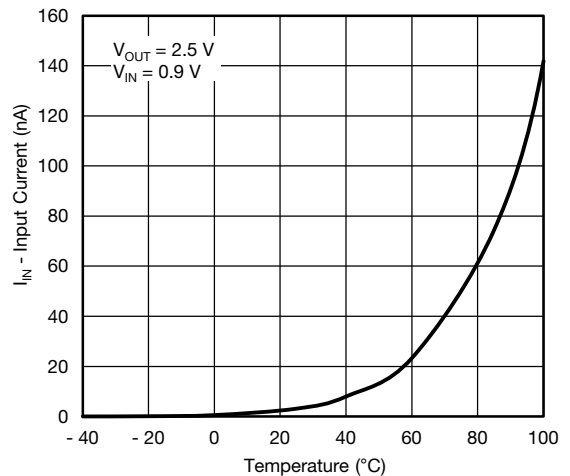
Reverse Blocking Current vs. Temperature
